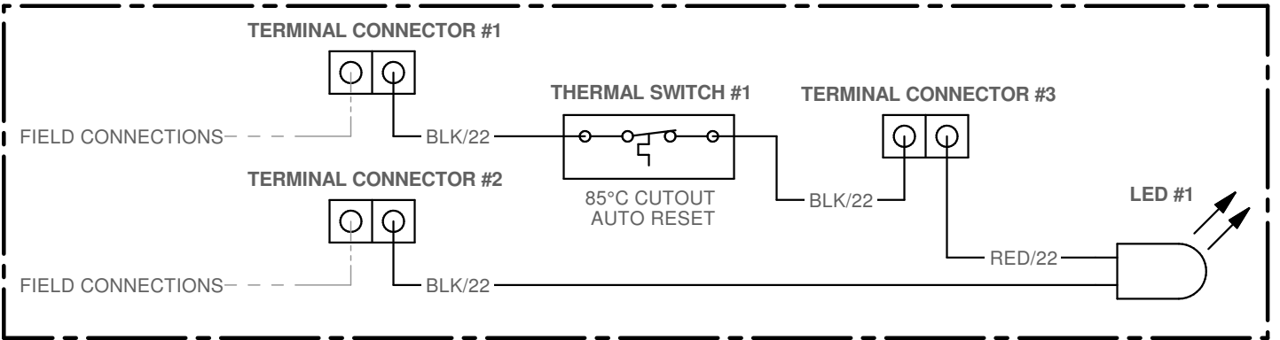
ELECTRICAL DIAGRAM TRIMLESS VERSION ONLY
