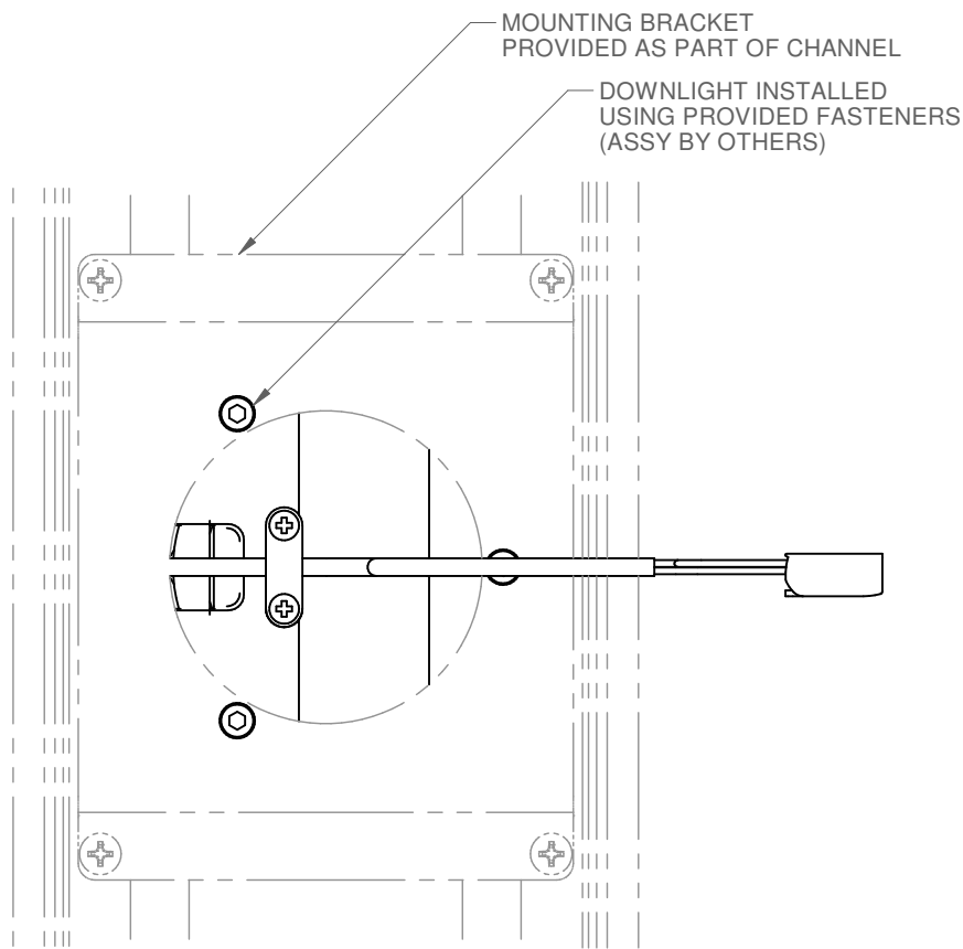
TOP VIEW FLUSH CHANNEL
