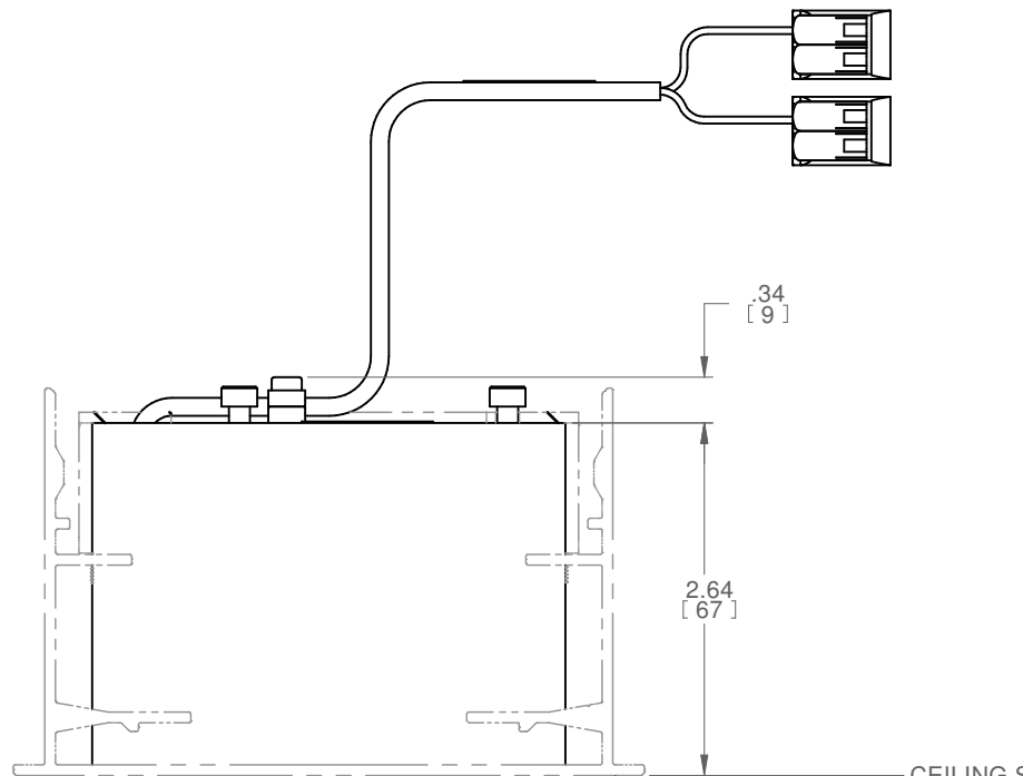
END VIEW FLUSH CHANNEL
