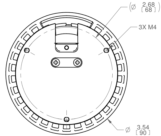
TOP VIEW FLUSH CHANNEL
