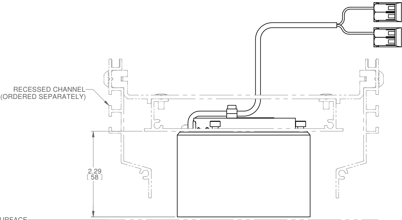
END VIEW RECESSED CHANNEL
