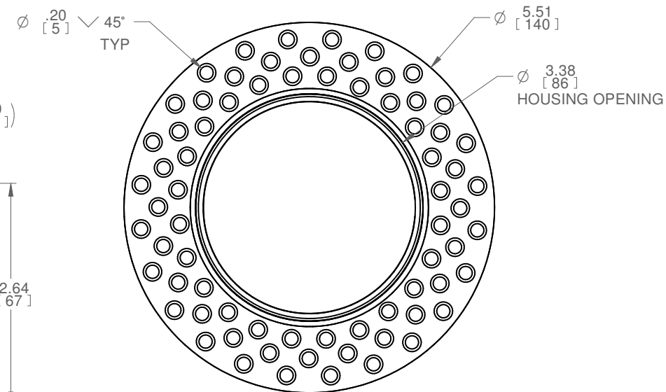
BOTTOM VIEW TRIMLESS
