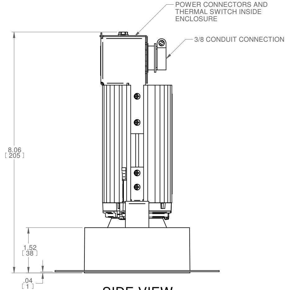
SIDE VIEW TRIMLESS
