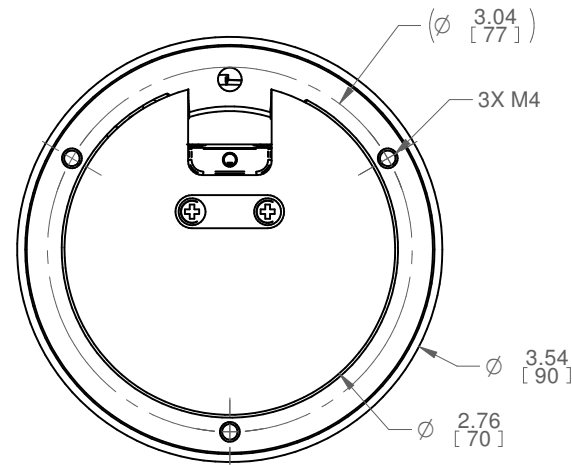
TOP VIEW RECESSED CHANNEL
