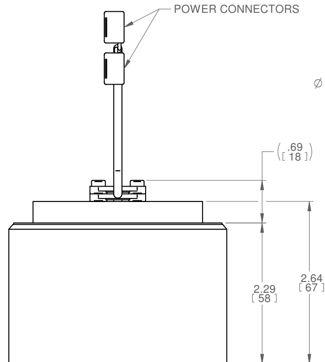
SIDE VIEW RECESSED CHANNEL
